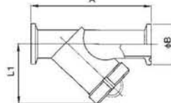
Clamp End
