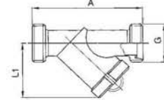
Thread End
