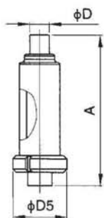
Weld End
