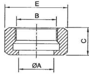
3A Hexagonal Nut 3A-13H
